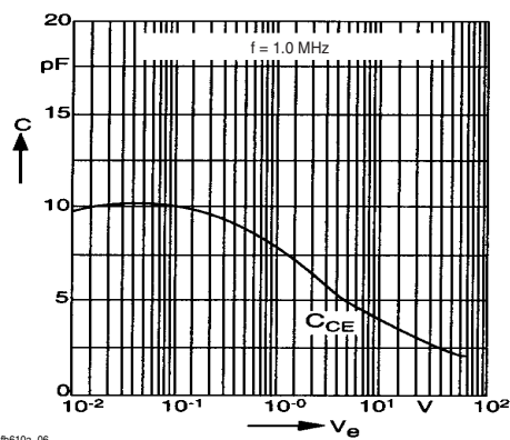
Figure 6. Transistor Capacitance (typ.) vs. Collector-Emitter Voltage
