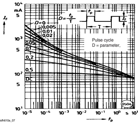
Figure 7. Permissible Pulse Handling Capability Forward Current vs. Pulse Width
