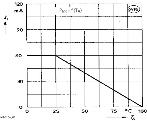
Figure 8. Permissible Power Dissipation vs. Temperature
