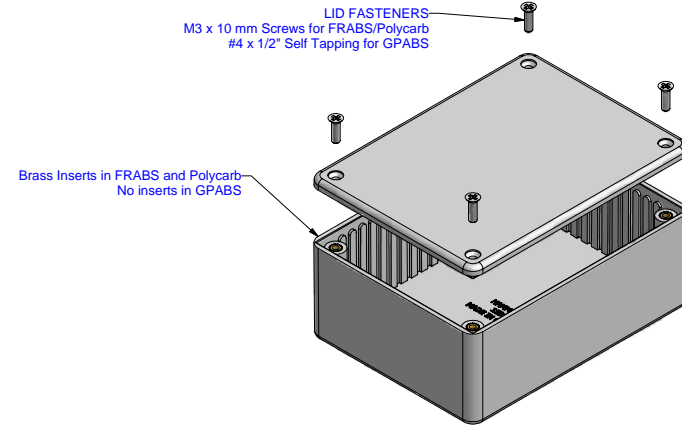
EXPLODED VIEW OF ASSEMBLY
