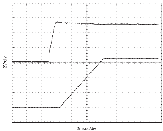
Power-Up From VIN (VIN = 5V, VOUT = 3.3V/10A, CIN = 220µF, No External COUT)
