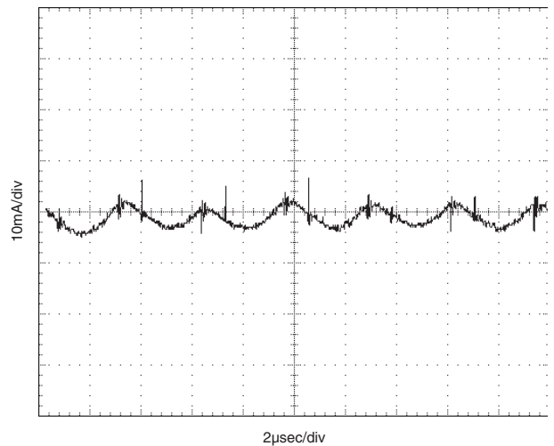
Input Reflected Ripple Current (VIN = 5V, VOUT = 3.3V/10A, Input Filter = 220µF/12µH/33µF, COUT = NA)
