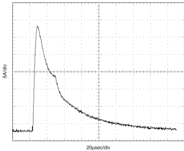
Input Reflected Ripple Current (VIN = 5V, VOUT = 3.3V/10A, CIN = 220µF, No External COUT)
