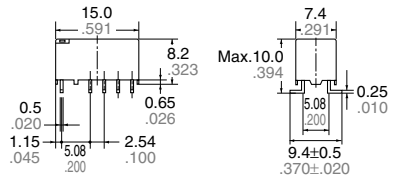
2 coil latching
