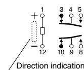
2 coil latching (Reset condition)
