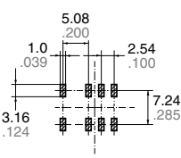
Suggested mounting pad
