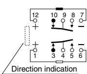
2 coil latching (Reset condition)
