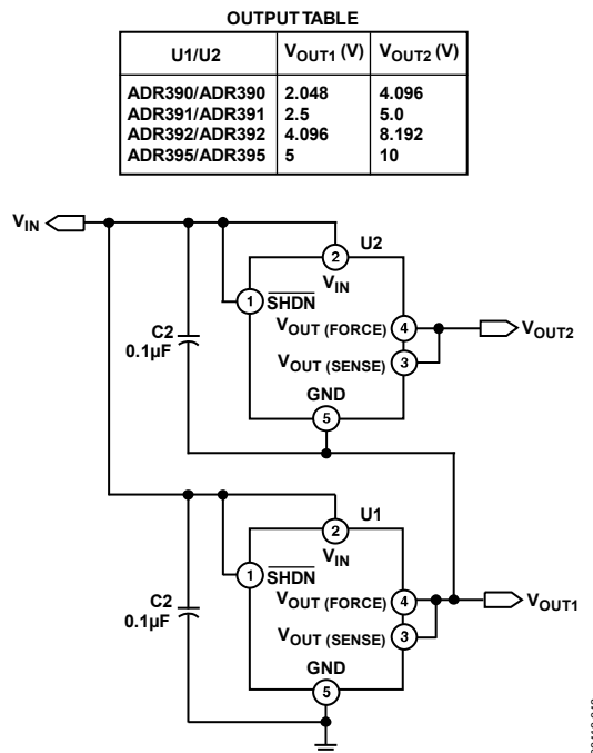
Figure 41. Stacking Voltage References with the ADR390/ADR391/ADR392/ADR395
