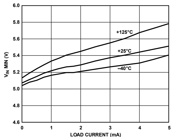
Figure 21. ADR395 Minimum Input Voltage vs. Load Current
