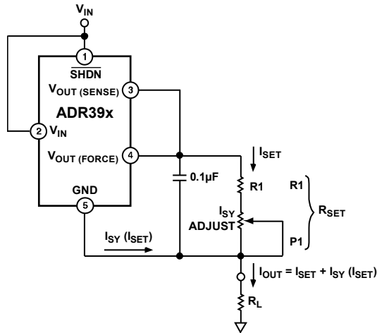
Figure 43. A General-Purpose Current Source
