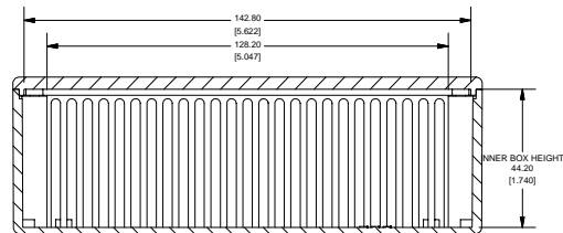
SECTION C-C SCALE 3 / 4
