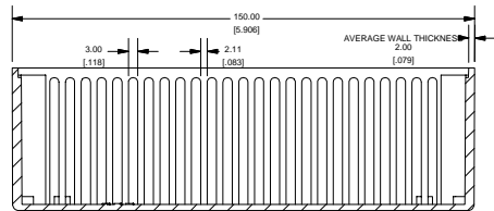
SECTION A-A SCALE 3 / 4
