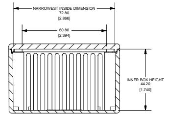
SECTION D-D SCALE 3 / 4
