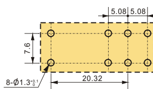
Wiring Diagrams (Bottom View)
