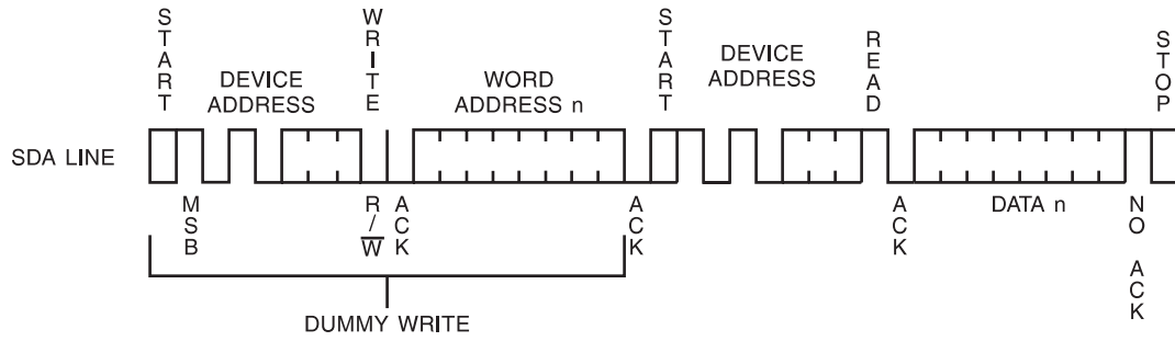
Figure 12. Random Read
