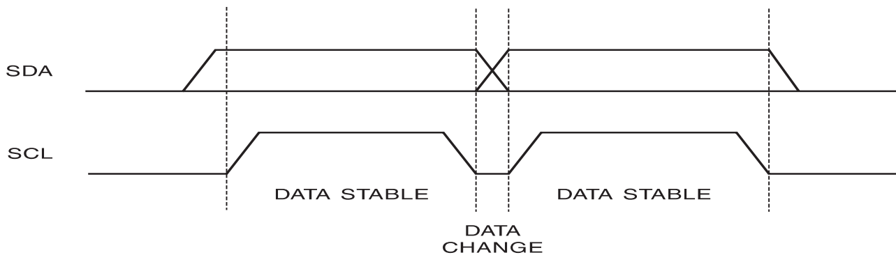
Figure 5. Data Validity
