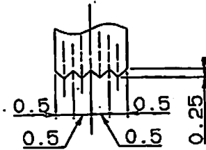
③"DETAILS (詳細)(5:1)
