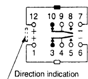
2 coil latching (Reset condition)
