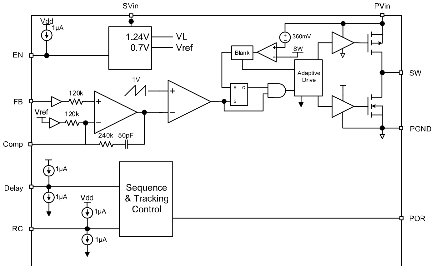
Figure 1. MIC22400 Block Diagram
