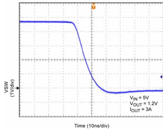
Switch Voltage (Falling Edge)
