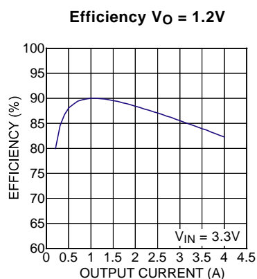
Figure 2. Efficiency Curve
