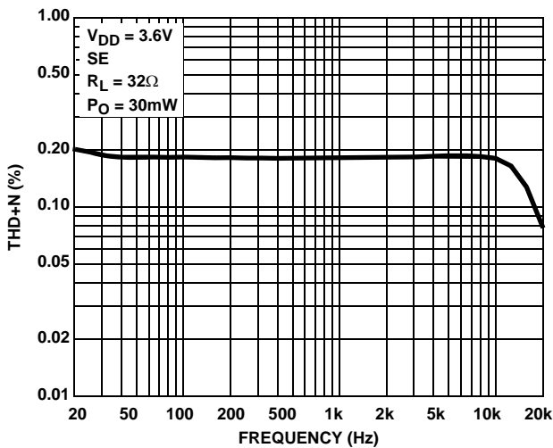
FIGURE 7. THD+N vs FREQUENCY
