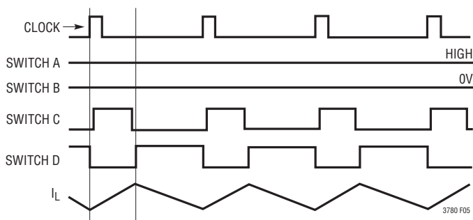
Figure 5. boost Mode ( V_{\text{IN}} < V_{\text{OUT}} )
