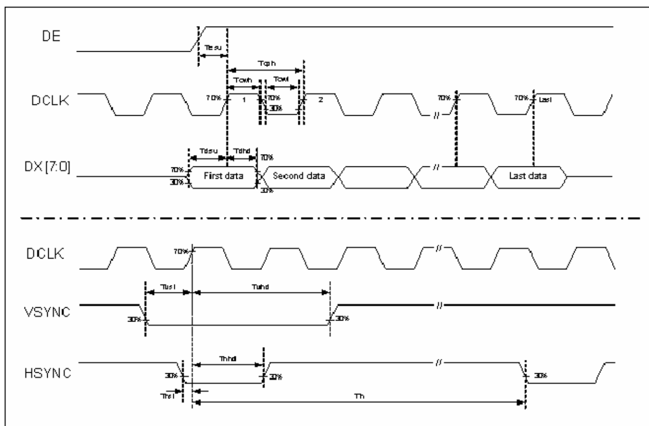
Clock and Data input waveforms
