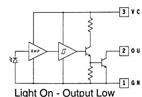
OPL551-OC (Open-Collector Output) Inverter
