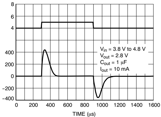
Figure 6. Line Transient Response
