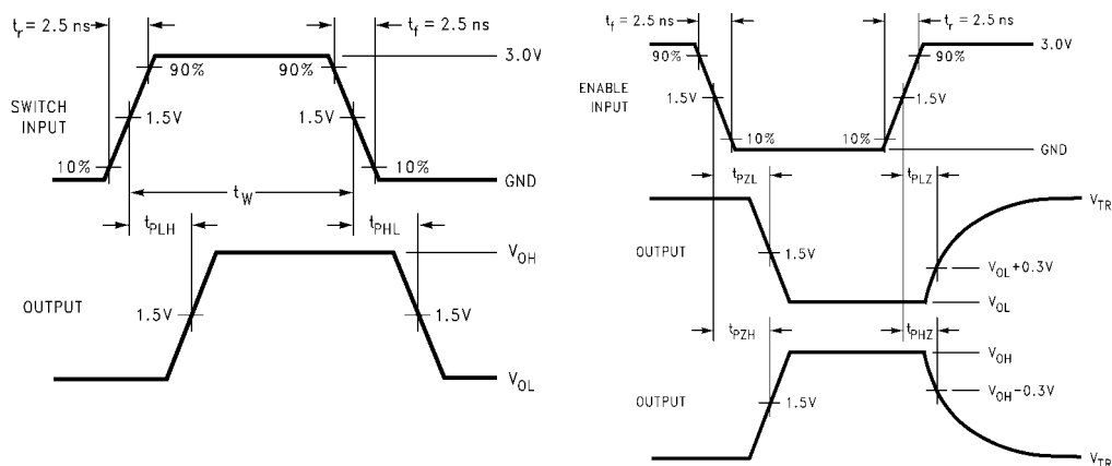
FIGURE 2. AC Waveforms
