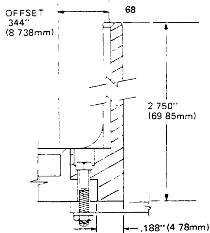
Offset Card Guide Field Assembled to -04 Type Insulator
