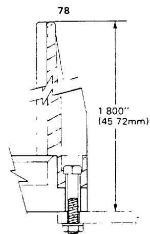
In-Line Card Guide Field Assembled to -04 Type Insulator
