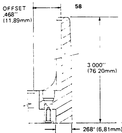
Offset Card Guides Factory Assembled with NO. 4-40 Threaded Insert
