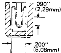
Cross Section Double Sided 090" (2.29mm) 200" (5.08mm)
