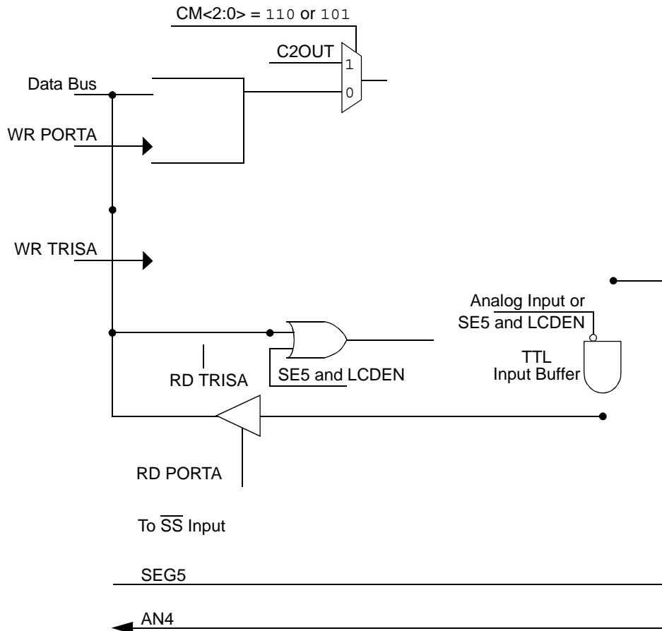
FIGURE 3-6: BLOCK DIAGRAM OF RA5/AN4/C2OUT/ \overline{SS} /SEG5
