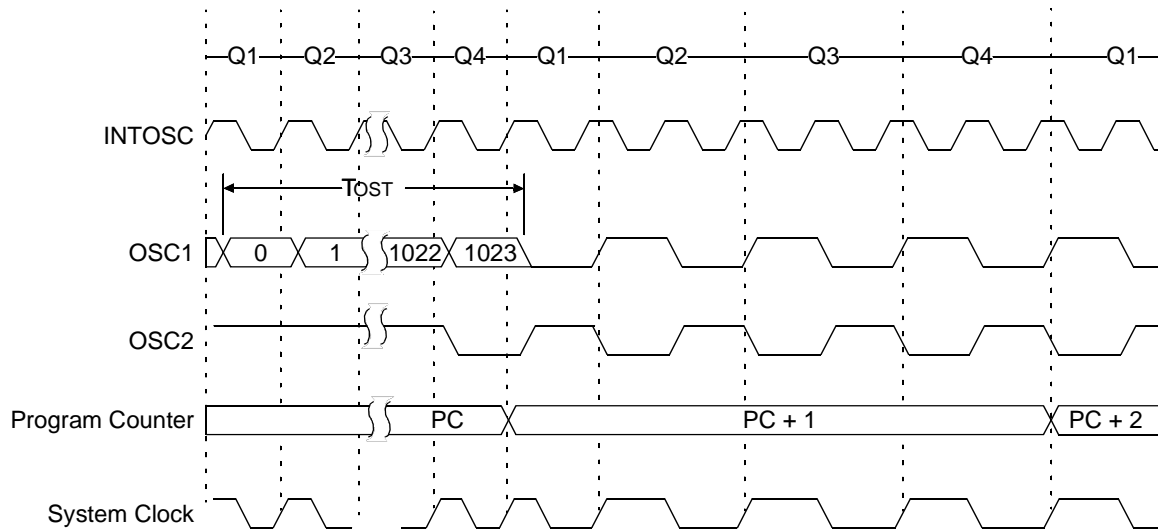
FIGURE 4-7: TWO-SPEED START-UP
