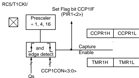
FIGURE 15-3: CAPTURE MODE OPERATION BLOCK DIAGRAM
