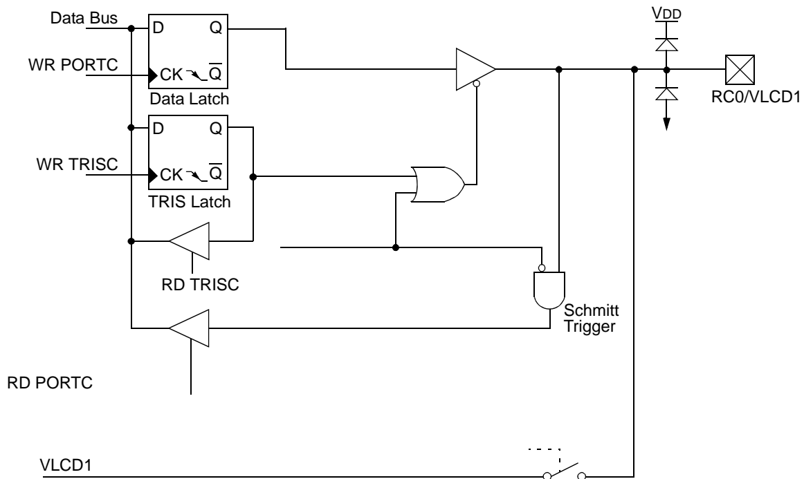
FIGURE 3-14: BLOCK DIAGRAM OF RC0/VLCD1
