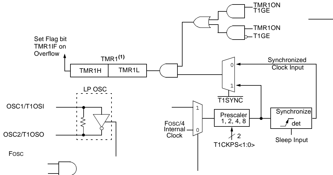
FIGURE 6-1: TIMER1 ON THE PIC16F917/916/914/913 BLOCK DIAGRAM
