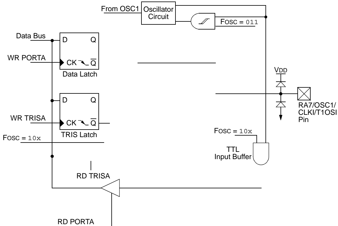
FIGURE 3-8: BLOCK DIAGRAM OF RA7/OSC1/CLKI/T1OSI
