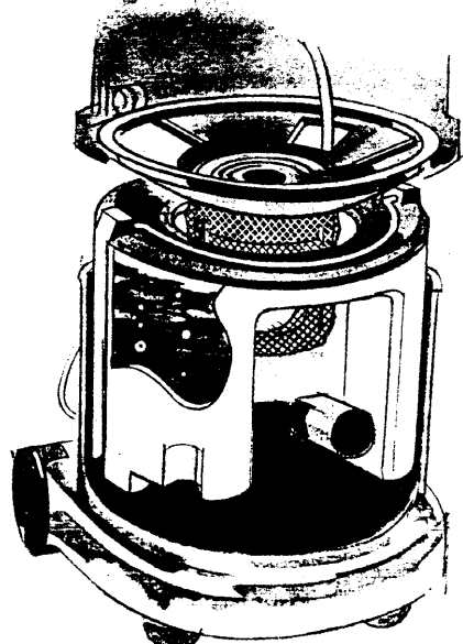
The dual clean-and-dirty liquid containers and safety float valve.
