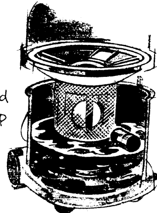
The dual clean-and-dirty liquid containers and safety float valve.
