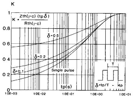
Fig. 7 : Relative variation of thermal transient impedance junction to case versus pulse duration. (ISOWATT220AB)
