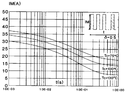
Fig. 5 : Non repetitive surge peak forward current versus overload duration. (Maximum values) (Per diode) (ISOWATT220AB)
