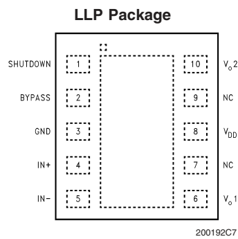
200192C7 Top View Order Number LM4890LD See NS Package Number LDA10B
