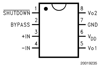
20019235 Top View Order Number LM4890M See NS Package Number M08A
