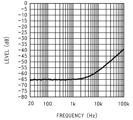
Power Supply Rejection Ratio (PSRR) @ A_V = 2
