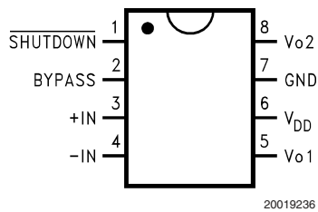
20019236 Top View Order Number LM4890MM See NS Package Number MUA08A
