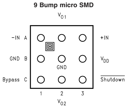
200192C1 Top View Order Number LM4890IBL, LM4890IBLX See NS Package Number BLA09AAB
