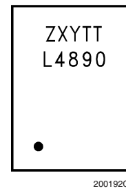
Top View Z - Assembly Plant Date Code (M for Malacca) XY - Digit Date Code TT - Die Traceability L4890 - LM4890LD
