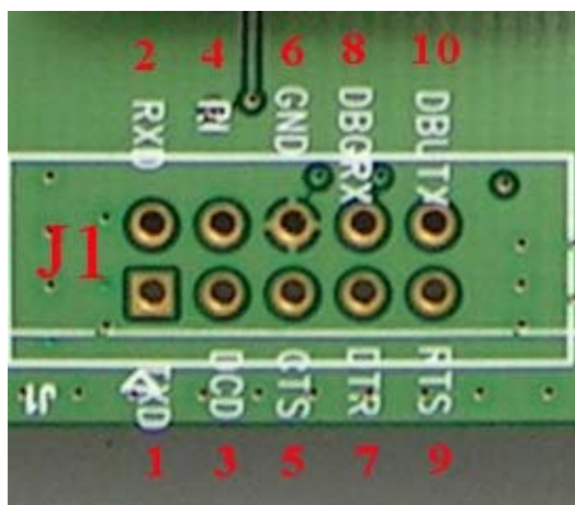
Figure 11: J1 Interface
