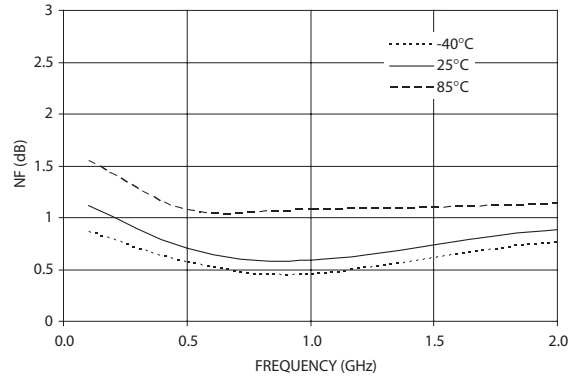
Figure 29. NF vs. Frequency (5V 15mA)
