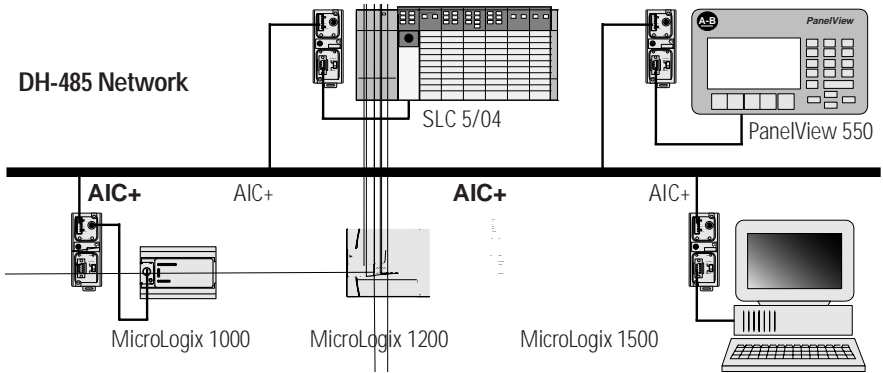
Example 1 - Local DH-485 Network with AIC+ (1761-NET-AIC) Interface
