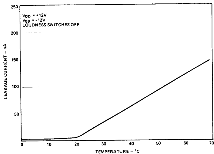
Figure 5. Loudness Switch Leakage Current vs. Temperature
