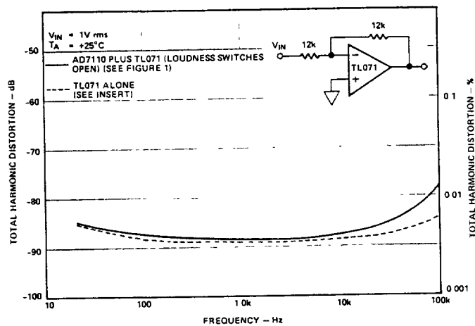
Figure 6. Total Harmonic Distortion vs. Frequency
