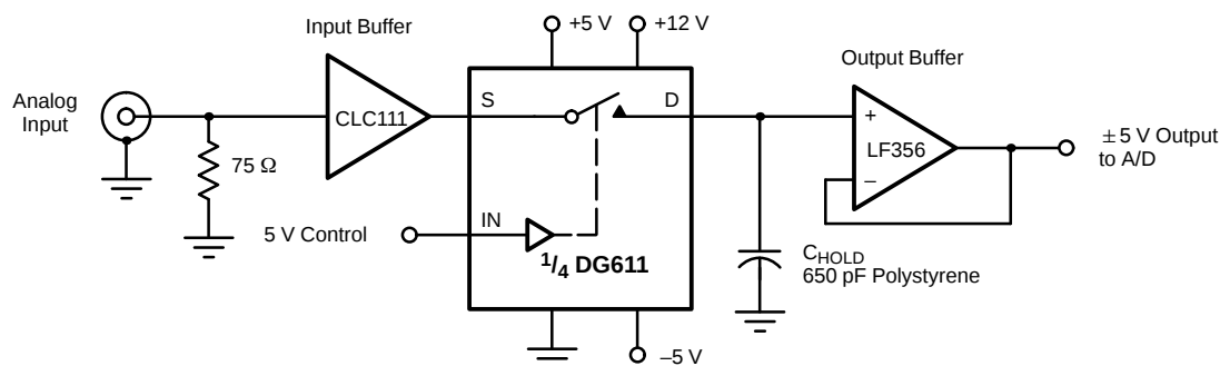
FIGURE 5. High-Speed Sample-and-Hold
