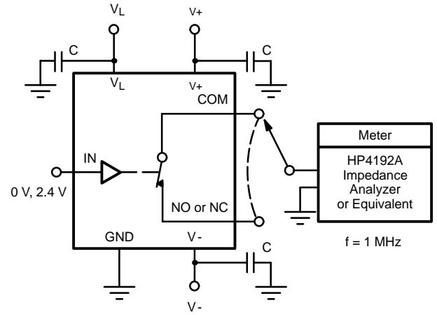
Figure 8. Source/Drain Capacitances
