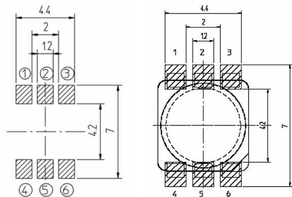
Land Pattern
