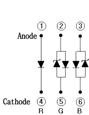
Circuit Diagram
