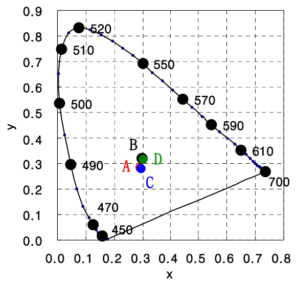
Chromaticity Diagram
