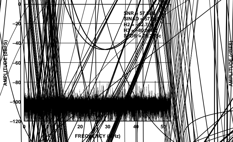
Figure 4. Frequency Response, A_{in} = 0.8 \text{ MHz} at -0.5 \text{ dBFS} ( -105 \text{ Grade} )
