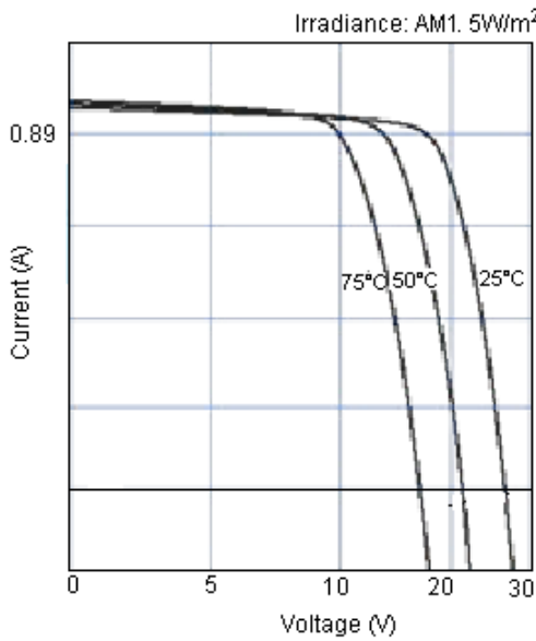
Current-voltage characteristics of photovoltaic Module SP15 at various cell temperatures
