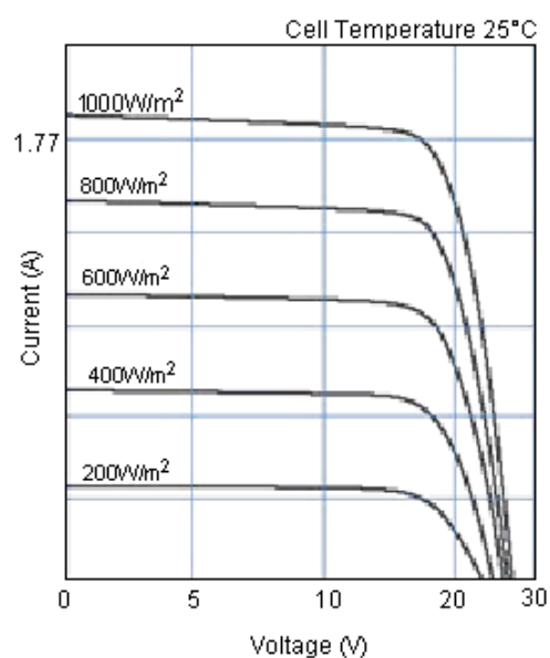
Current-voltage characteristics of photovoltaic Module SP30 at various irradiance levels
