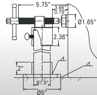
Model VSC15 Weight: 5.6 lbs (2.6 kg)
