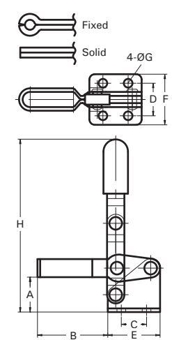
Model GH-12050 Shown
