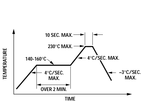
Figure 6. Recommended reflow soldering profile.
