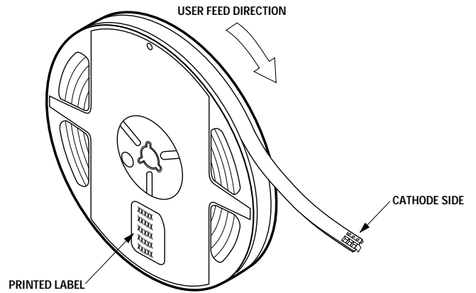
Figure 9. Reeling orientation.
