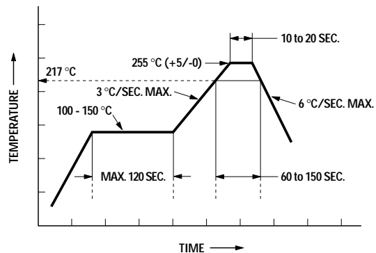
Figure 7. Recommended Pb-free reflow soldering profile.
