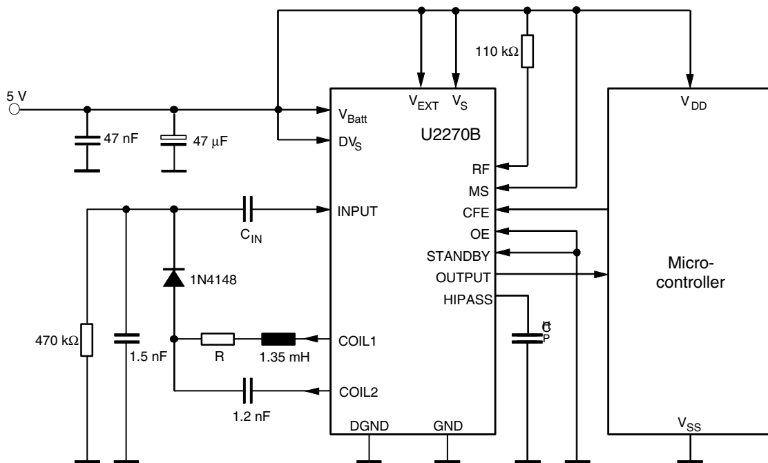
Figure 4-1. Application Circuit 1
