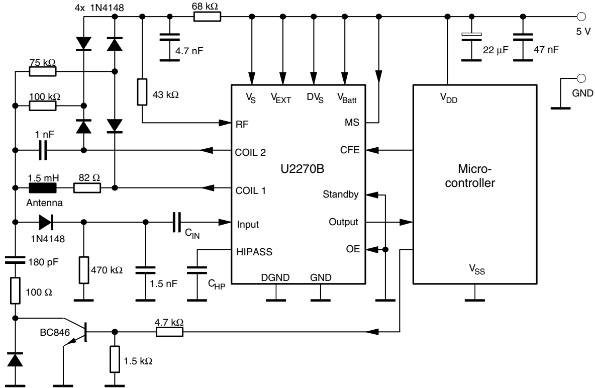
Figure 4-3. Application Circuit 3
