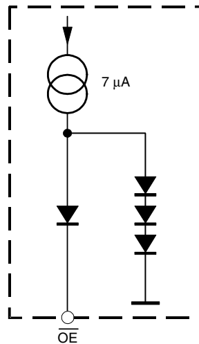
Figure 3-8. Equivalent Circuit of Pin OE
