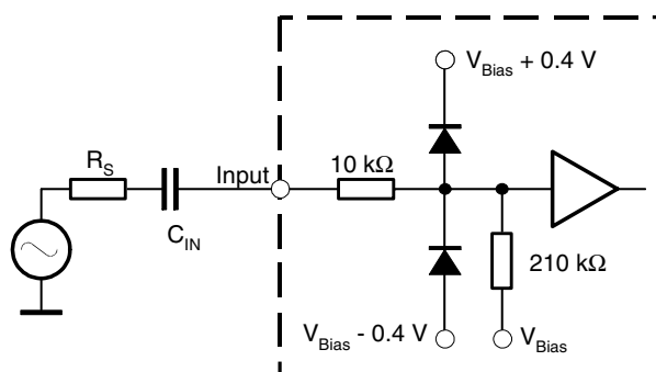
Figure 3-6. Equivalent Circuit of Pin Input
