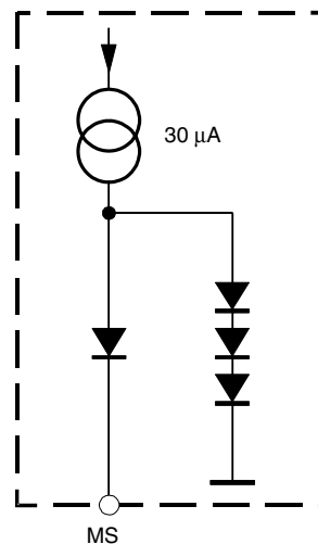
Figure 3-9. Equivalent Circuit of Pin MS
