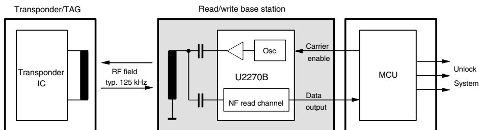
Figure 1-1. System Block Diagram
