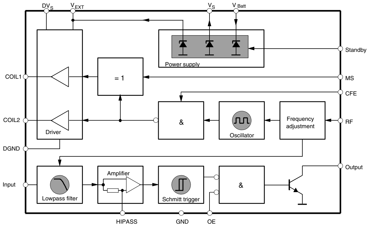
Figure 1-2. Block Diagram
