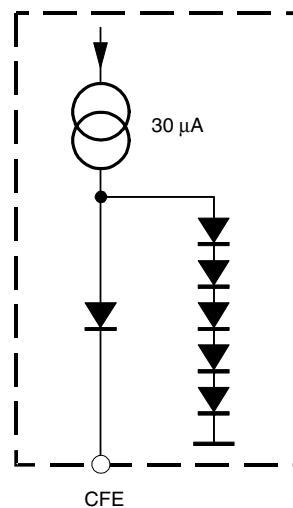
Figure 3-10. Equivalent Circuit of Pin CFE
