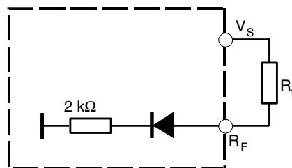
Figure 3-5. Equivalent Circuit of Pin R_F
