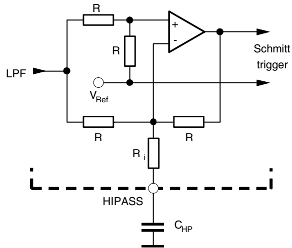
Figure 3-7. Equivalent Circuit of Pin HIPASS
