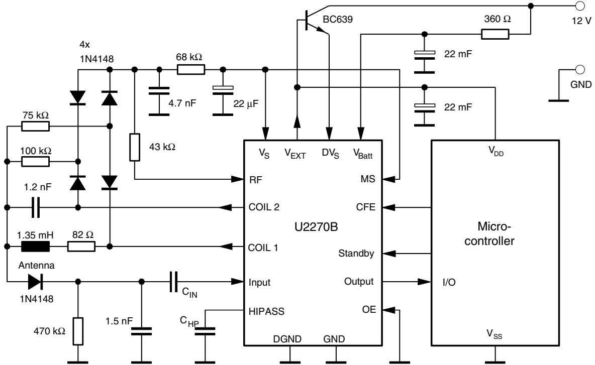
Figure 4-2. Application Circuit 2
