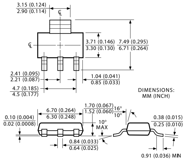
SOT-223 (S)
