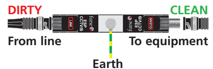
Series connection for ESP CCTV/B.
