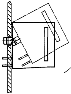
JACK DISMOUNT METHOD DETAIL A NOTE 5
