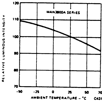
Fig. 9. Relative Luminous Intensity vs. Temperature
