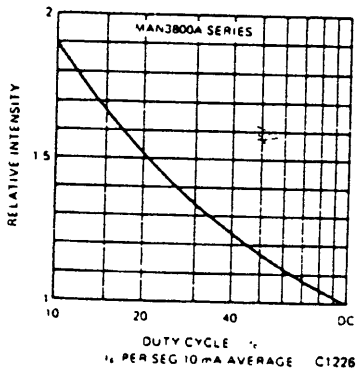
Fig. 17. Luminous Intensity vs. Duty Cycle
