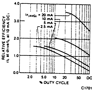
Fig. 11. Relative Efficiency vs. Duty Cycle
