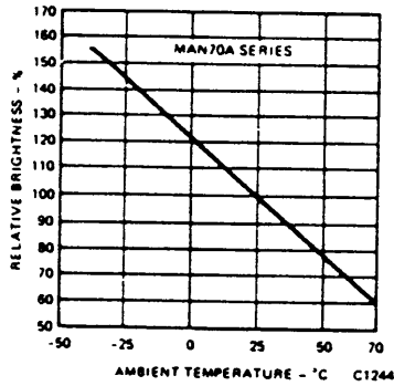
Fig. 7. Relative Luminous Intensity vs. Temperature
