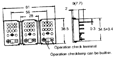
PY14-3 (for 4PDT) with operation check terminal
