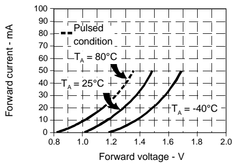
Fig. 3 IRED Forward Bias Characteristics gra_073.ds4
