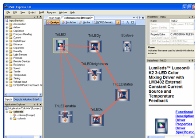
Figure 3. PSoC Express
