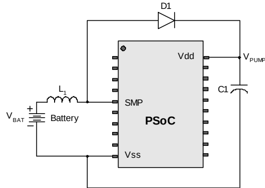
Figure 5. Basic Switch Mode Pump Circuit
