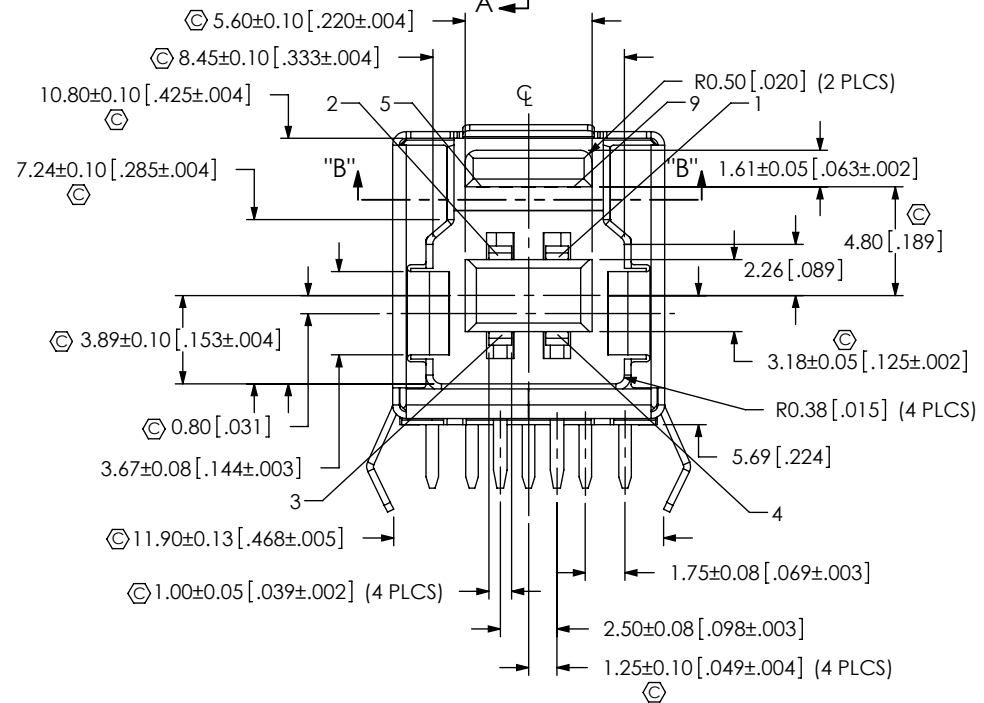
FIG. 1 (USB3-B-S-X-TH SHOWN)
