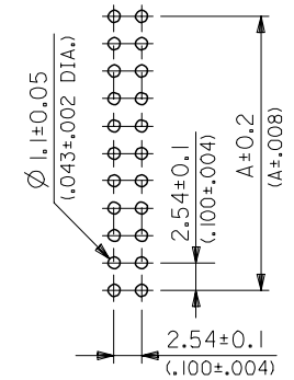
RECOMMENDED P.C.BOARD PATTERN
