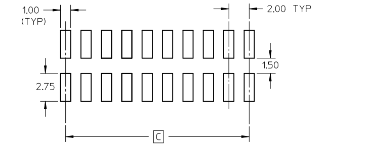
RECOMMENDED PCB PATTERN
