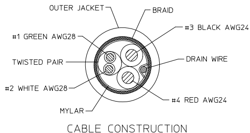
CABLE CONSTRUCTION
