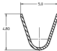
SECTION Z-Z CONDUCTOR CRIMP 12 AWG
