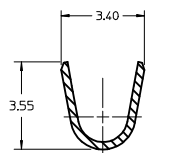
SECTION Z-Z CONDUCTOR CRIMP 14/16 AWG
