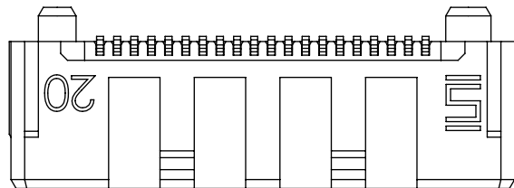
FIG 1 (LSHM-1XX-XX.X-DV-A-N-X-TR SHOWN)
