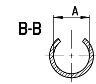
ISOLATIONSCRIMP GR. 18-16 INSULATION CRIMP SIZE 18-16
