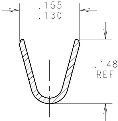
SECTION B-B SCALE 8:1
